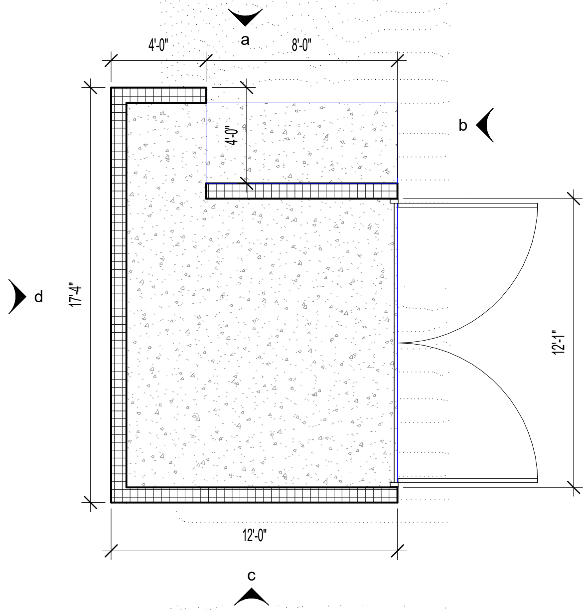
typical dumpster enlosure
