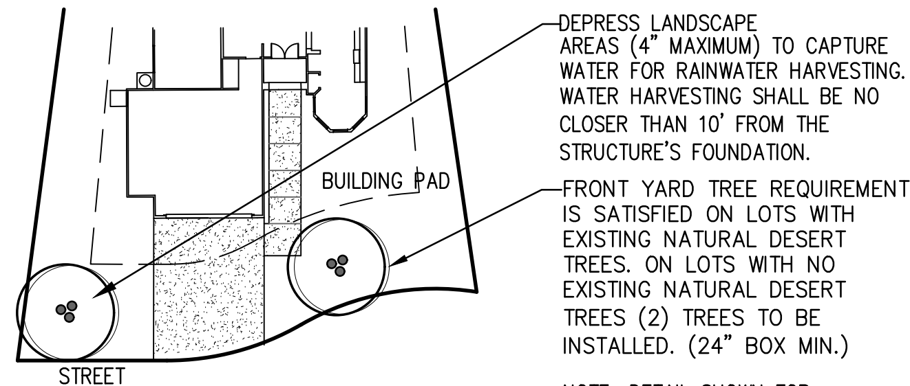
FRONT YARD PLANTING DETAIL SCALE: NTS
