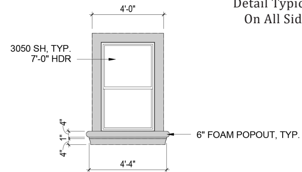
Window Detail
