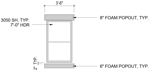
Window Detail
