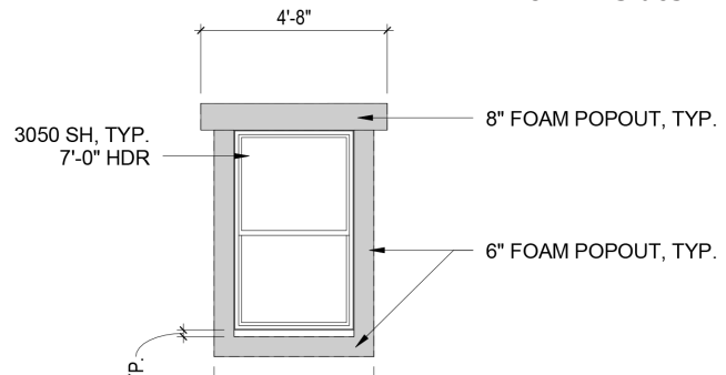
Window Detail
