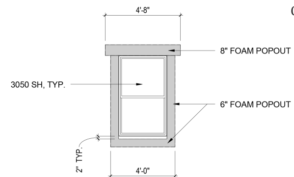
Window Detail
