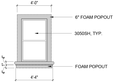
Window Detail
