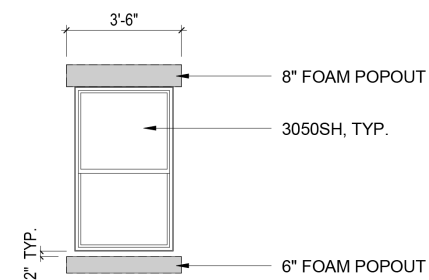
Window Detail
