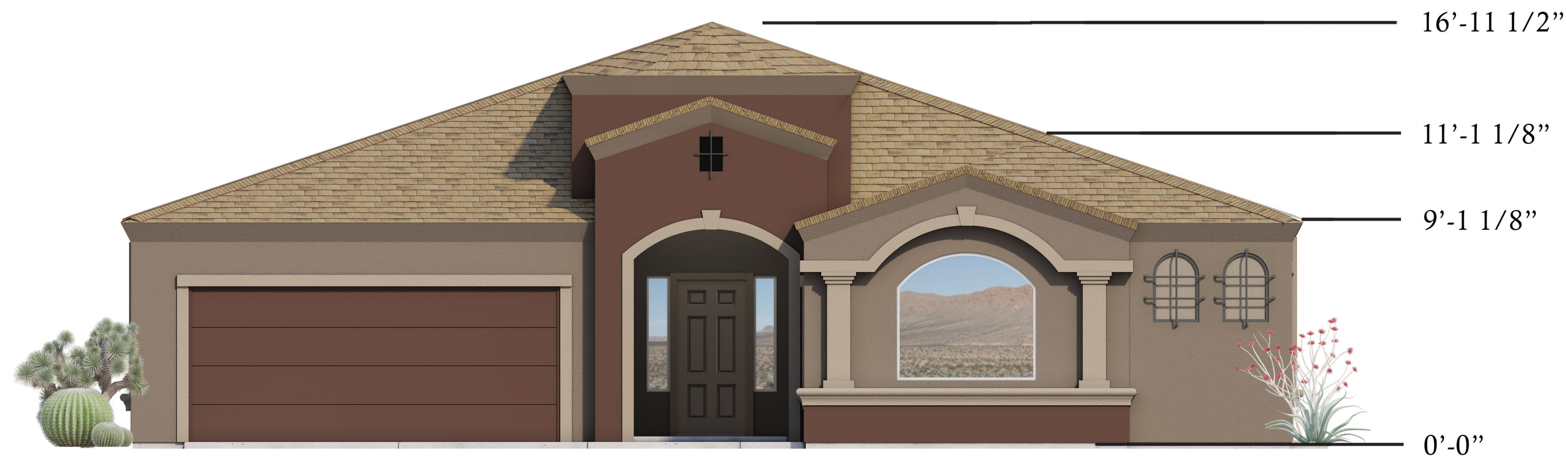
Front Elevation
