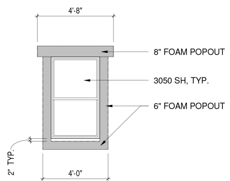
Window Detail
