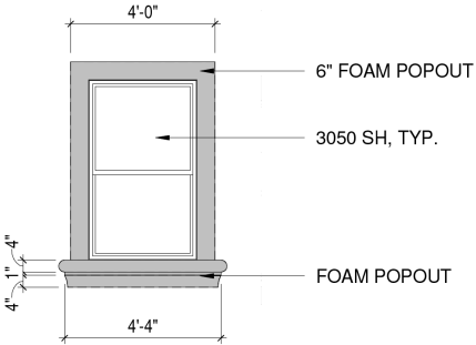
Window Detail
