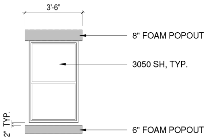
Window Detail
