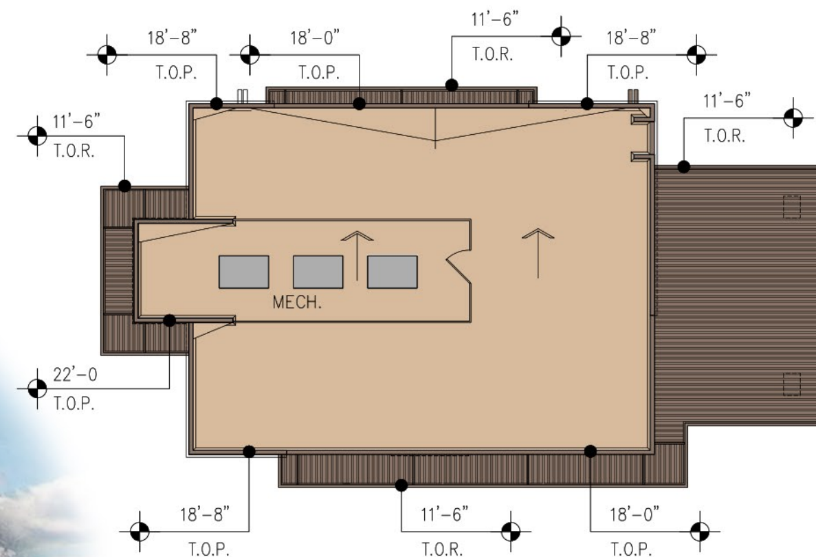
3 ROOF PLAN SCALE: 1/16" = 1'-0"
